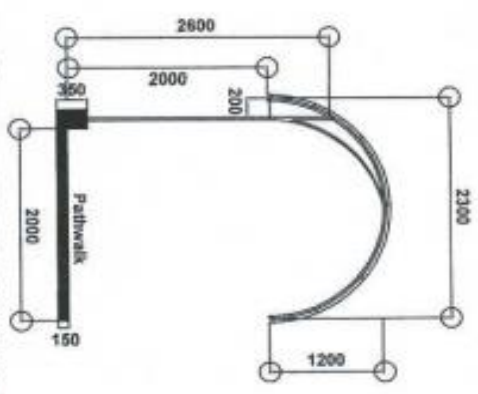
COVERED PATHWALK PLAN SCALE: NTS
