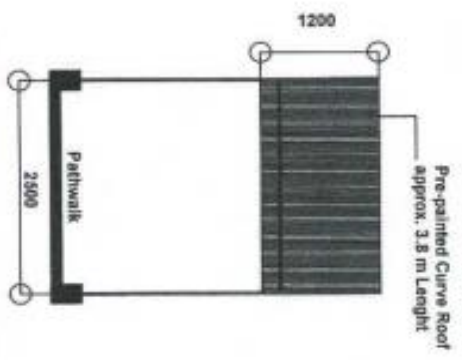
COVERED PATHWALK DETAILS SCALE: NTS
